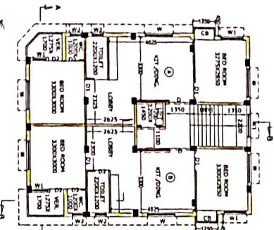
1ST, 2ND, & 3RD FL. PLAN
